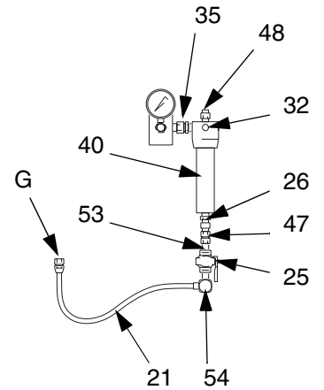
Catalyst Outlet Detail
