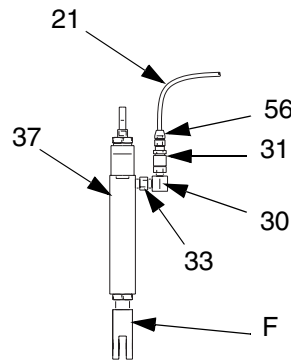
Catalyst Pump Detail
