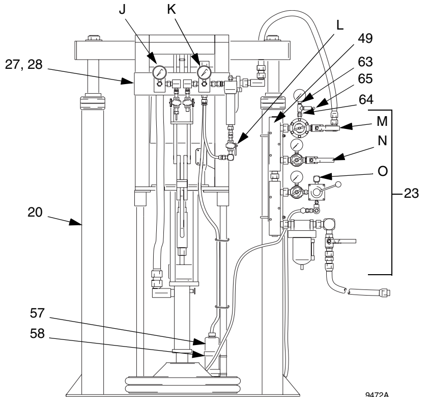
Catalyst Pump Detail
